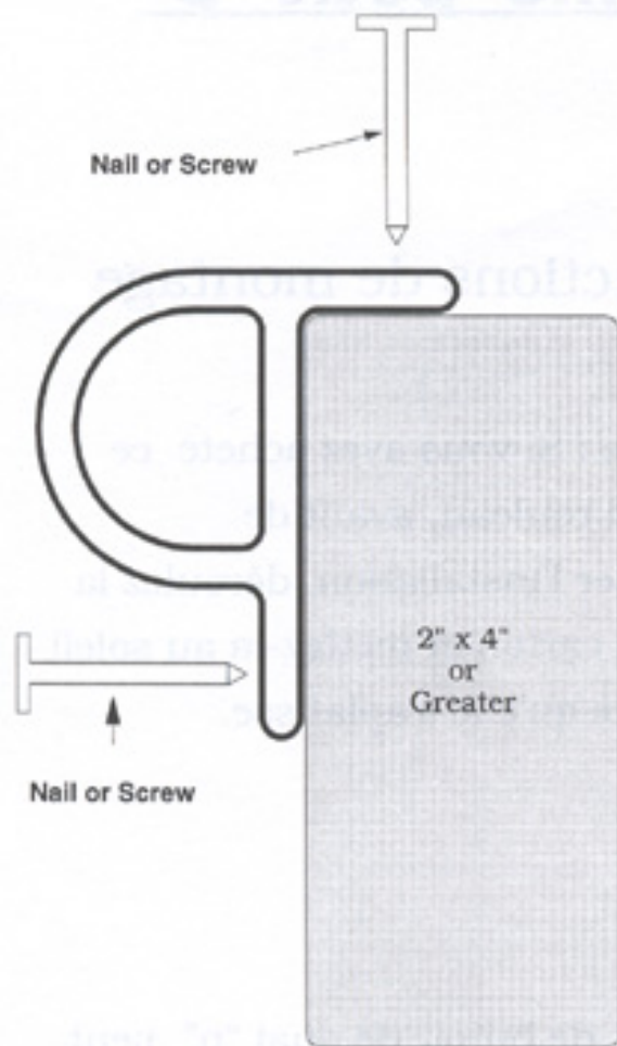
END VIEW
